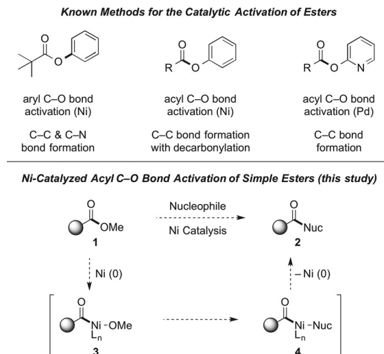
Figure 1. Known methods for the catalytic activation of esters and our approach for the activation of methyl esters (without decarbonylation).
